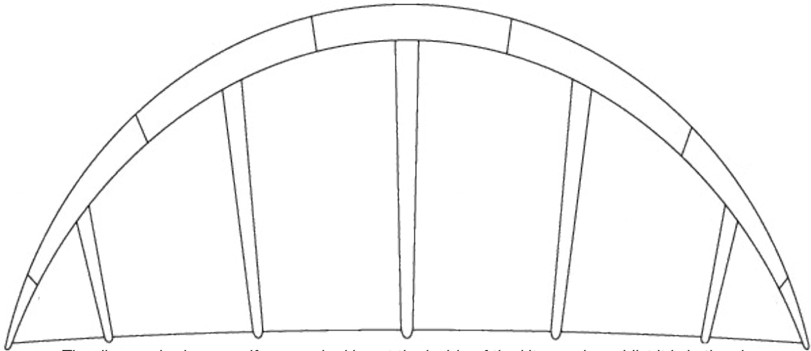
The diagram is shown as if you are looking at the inside of the kite or wing whilst it is in the air
